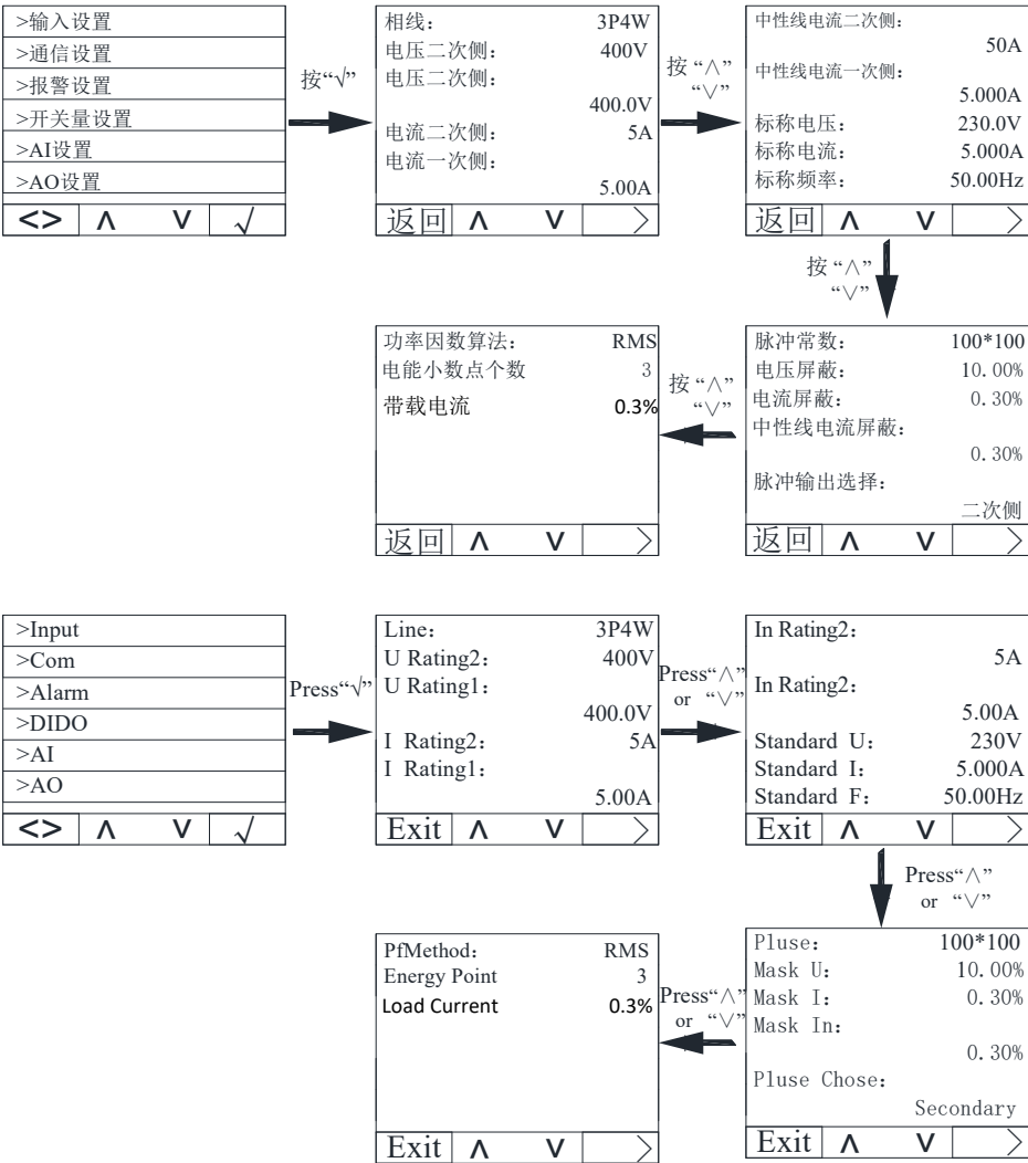
图 14 输入设置操作图 Figure 14 Enter the setup operation chart
