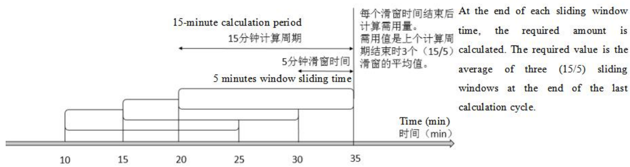
图 24 需量计算示意图 Figure 24 Schematic diagram of demand calculation
